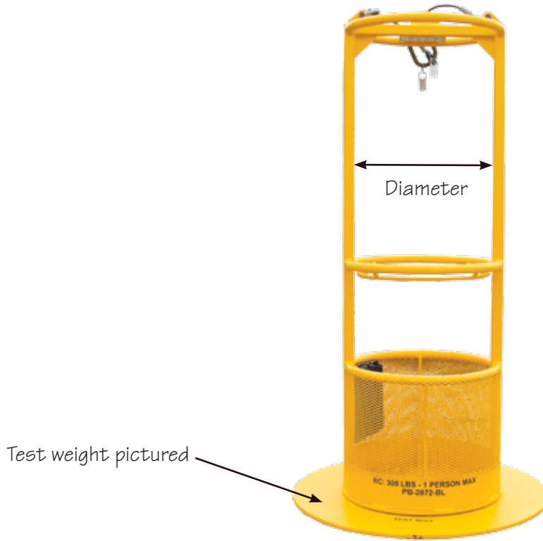
Model: PBR - Liftmax® Personnel Basket, Round
